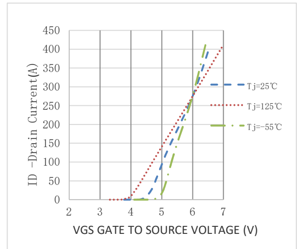
Figure 10. Transfer Characteristics
